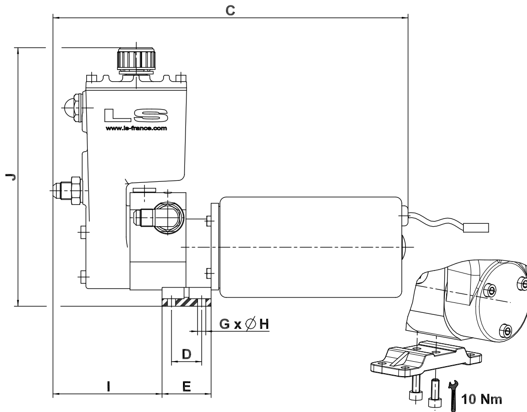
Ensembles linéaires Linear drives 32 ST 16 – 40 ST 16 50 ST 20 – 50 ST 203
